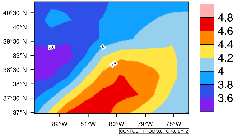
Yearly pr (mm/day) In 2020-2029 MIROC4h RCP45 - West Virginia
