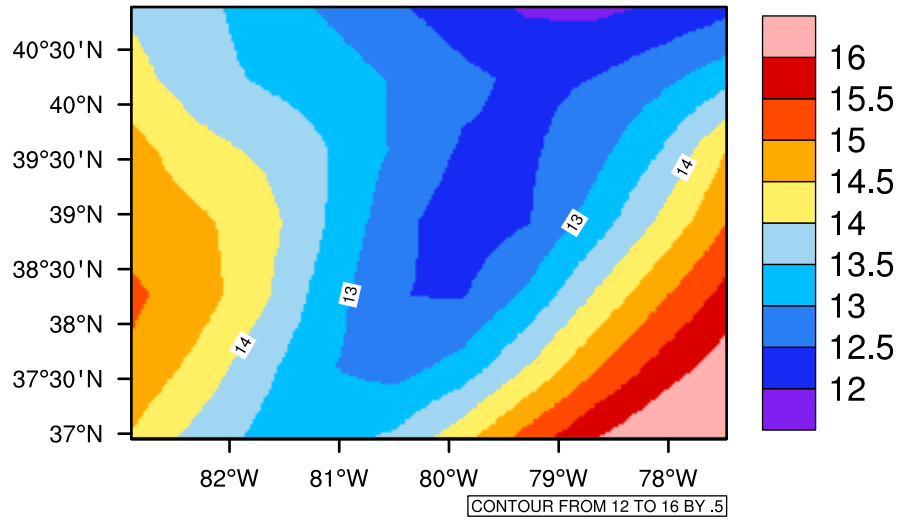
Yearly tas (c) In 2020-2029 MIROC4h RCP45 - West Virginia
