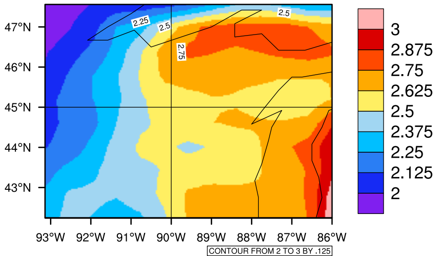
Yearly pr (mm/day) In 2020-2029 MIROC4h RCP45 - Wisconsin
