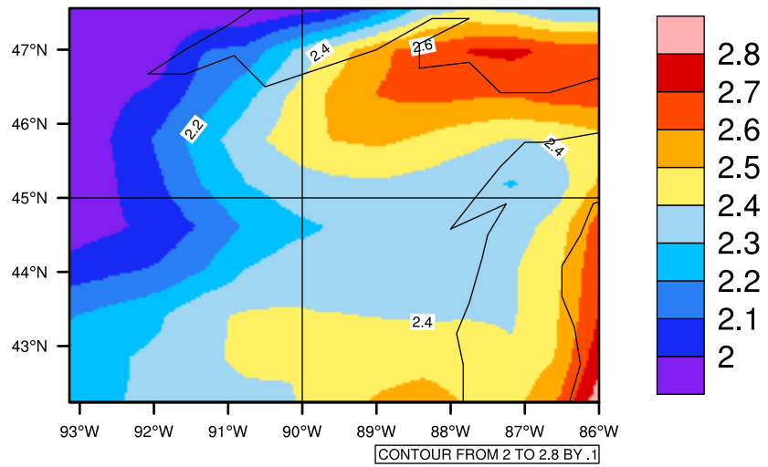
Yearly pr (mm/day) In 1975-2005 MIROC4h historical - Wisconsin
