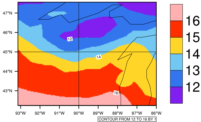
Yearly tasmax (c) In 1975-2005 MIROC4h historical - Wisconsin
