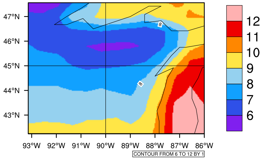
Yearly tasmin (c) In 2020-2029 MIROC4h RCP45 - Wisconsin
