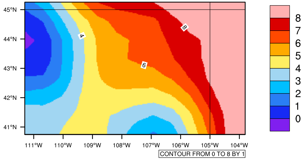
Yearly tas (c) In 1975-2005 MIROC4h historical - Wyoming
