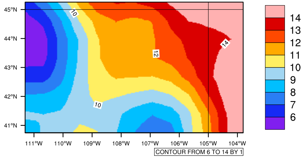
Yearly tasmax (c) In 1975-2005 MIROC4h historical - Wyoming
